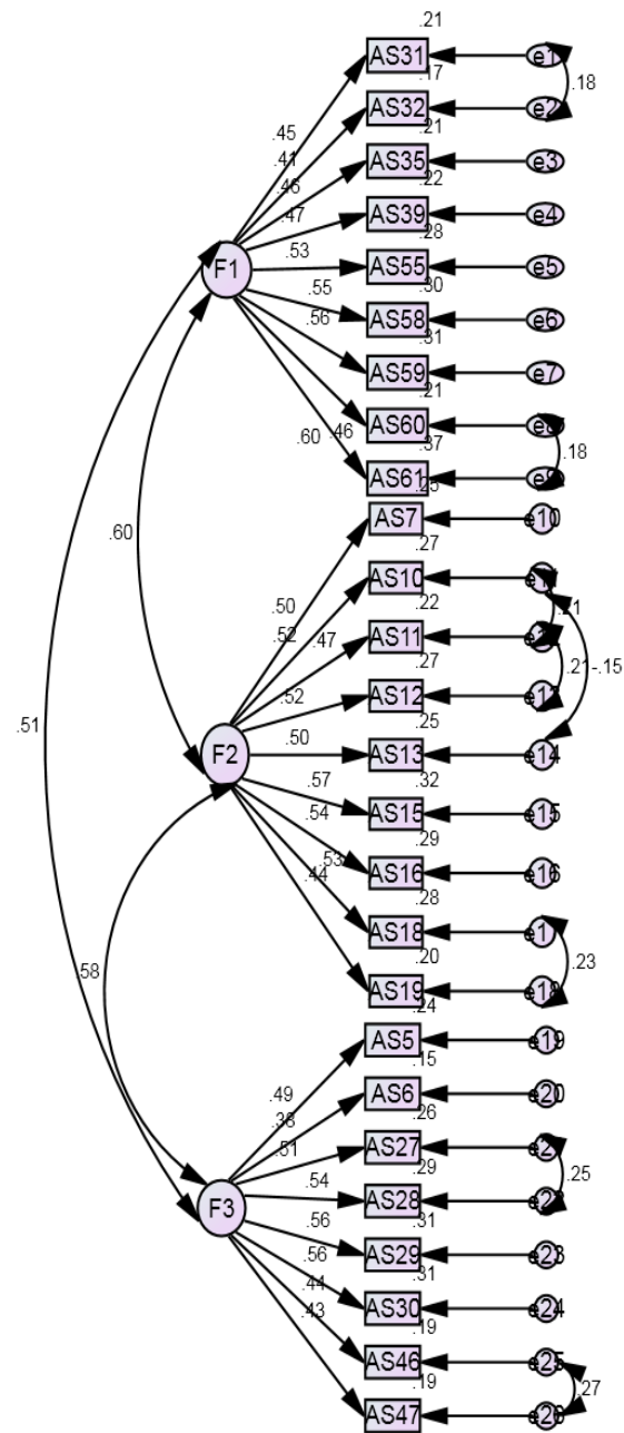
Figure 1. Measurement model of Academic Stress Scale for University Students
